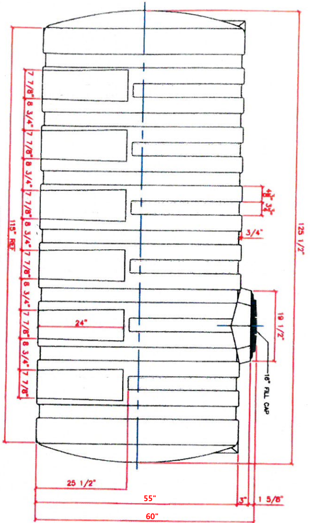
VIEW A
